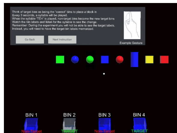
Figure 3: Tutorial
